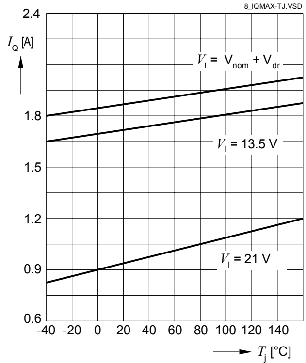
Output Current Limit I_{Qmax} versus Junction Temperature T_j
